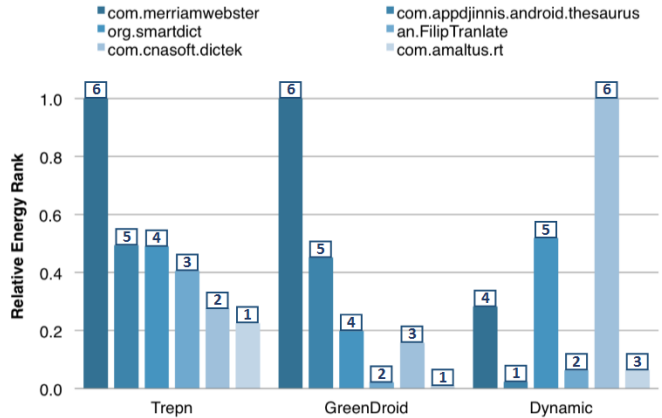
Fig. 5: Visualization of rankings provided by Trepn, EcoDroid, and dynamic approach.
