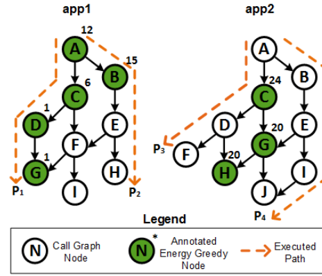
Fig. 3: Call graph and executed paths of two Android apps.
