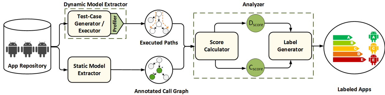
Fig. 2: EcoDroid Framework.
